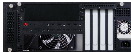
Rear View
